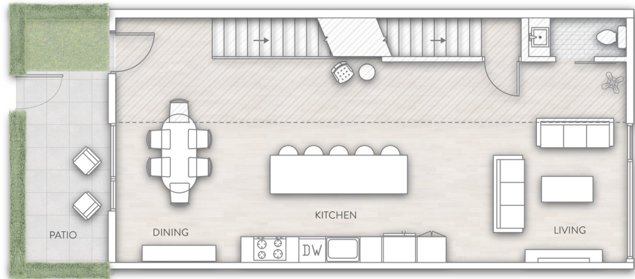
UNIT D - LEVEL 1
